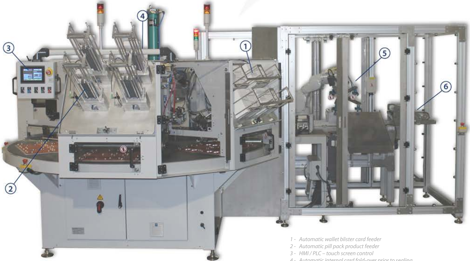
FAB/PH6-1824-CS - automatic rotary heat seal & cold seal machine for pharmaceutical wallet packages with internal and external card fold-over
